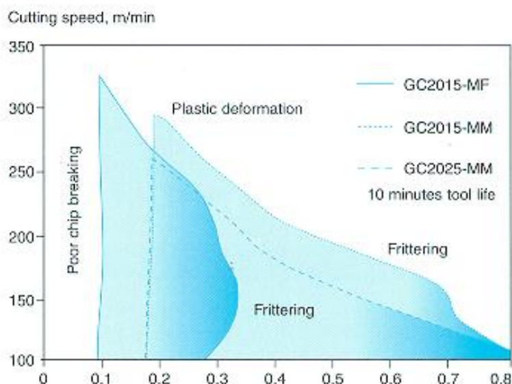
Figure 1. Machining chart Sandvik Sanmac 304L and 316L.
